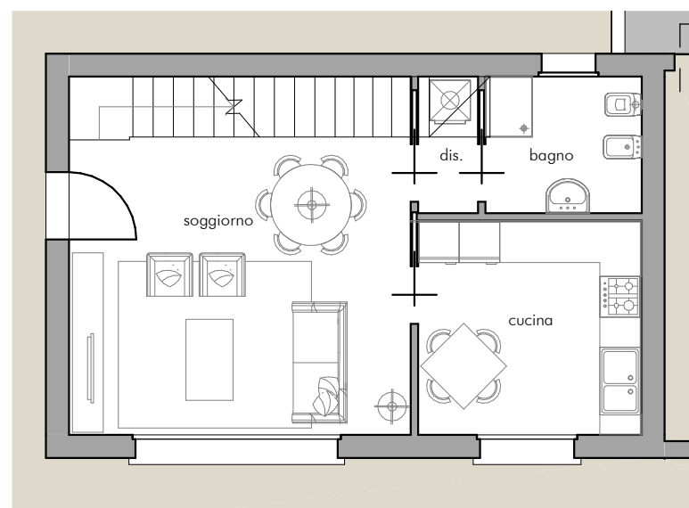
Piano terra 1:100
